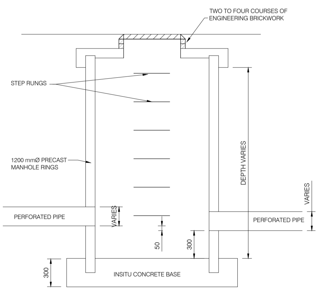
TYPICAL PRECAST RING MANHOLE, DEPTH TO SOFFIT 0-3 m SCALE 1:25
