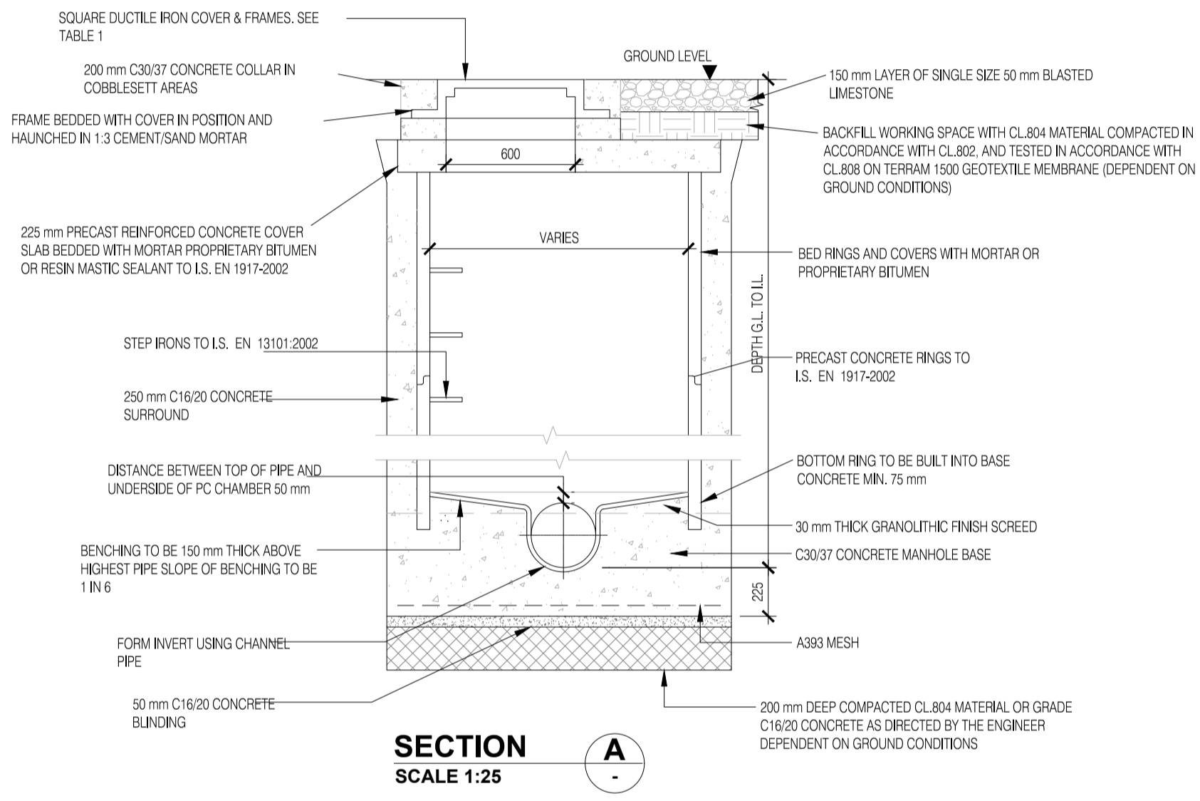
TYPICAL PRECAST RING MANHOLE, DEPTH TO SOFFIT 0-3 m SCALE 1:25
