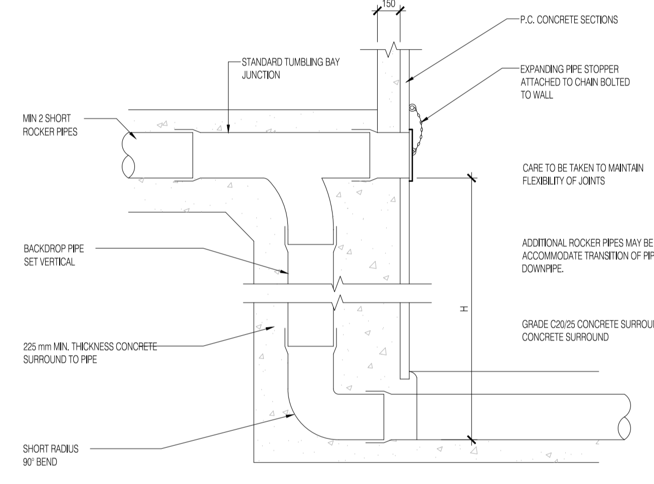
TYPICAL VERTICAL BACKDROP DETAIL SCALE 1:25 (STEEPER GRADIENTS ARE PREFERRED TO THE USE OF BACKDROPS)
